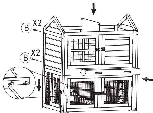
6. Fix the ramps and the top back panel with then tray and the partition.
