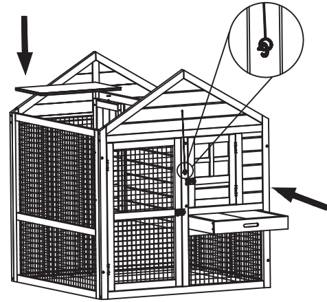
4. Insert the shelf and tray.
