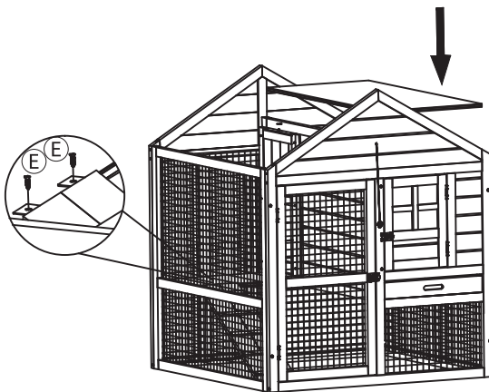
5. Fix the ramp.
