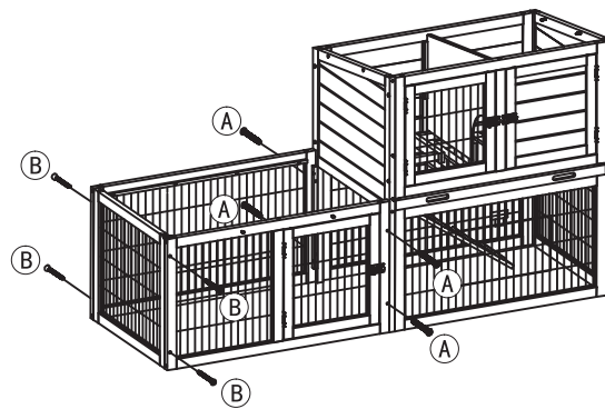
6. Fix the enclosure front & back panel and the enclosure side panel .
